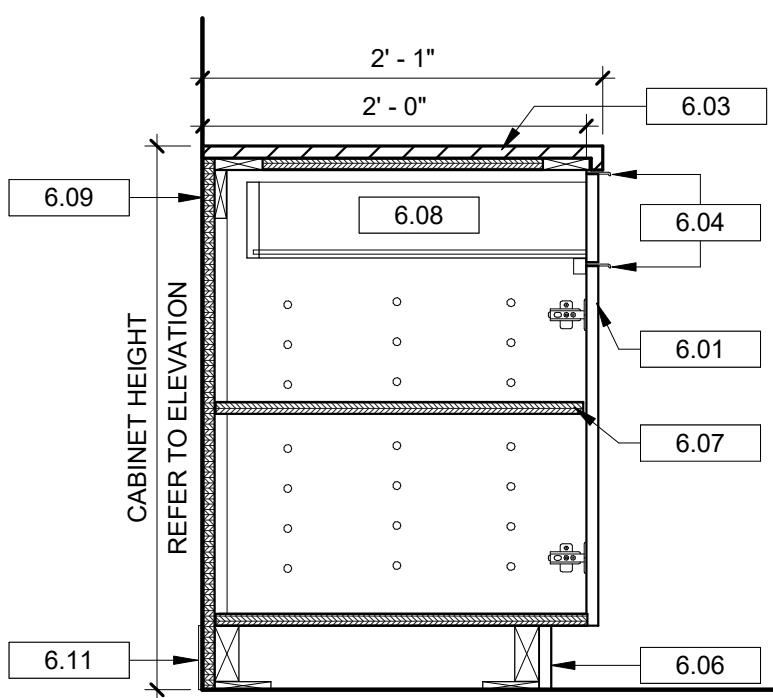
4 SECTION AT TYPICAL BASE CABINET A11.02 1" = 1'-0"
