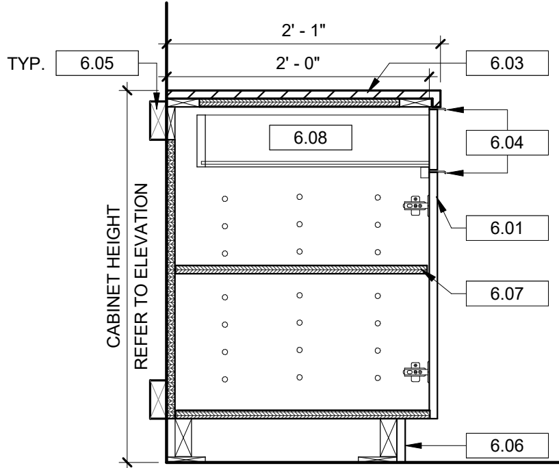
2 SECTION AT BASE CABINET AT WALL A11.02 1" = 1'-0"
