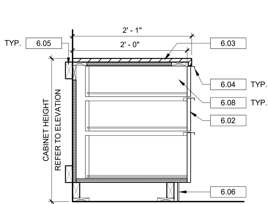
1 SECTION AT 3 DRAWER BASE AT WALL A11.02 1" = 1'-0"
