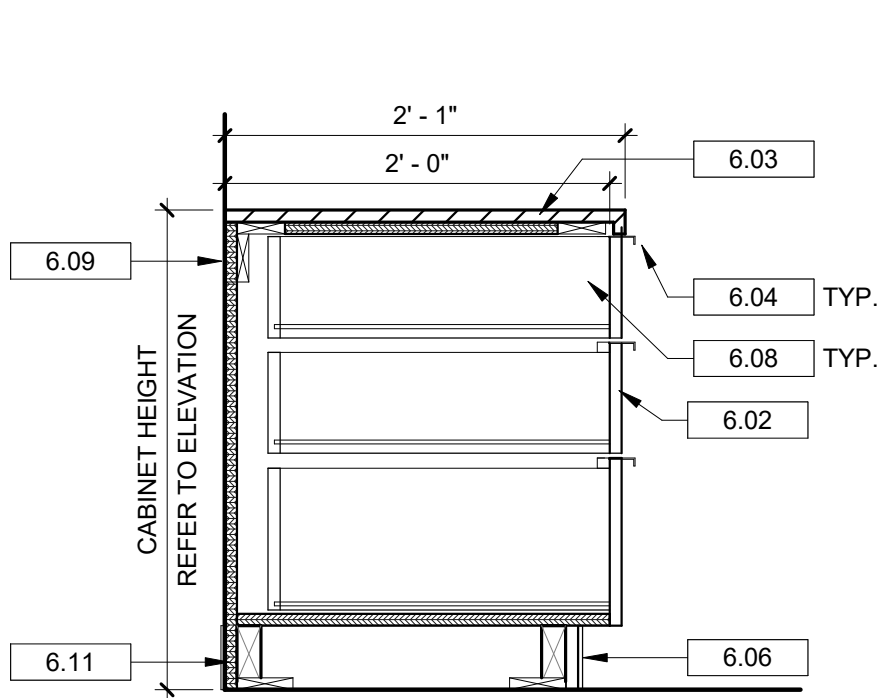
3 SECTION AT TYPICAL 3 DRAWER BASE A11.02 1" = 1'-0"
