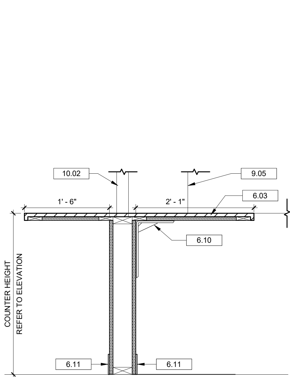
5 SECTION AT LOBBY COUNTER A11.02 1" = 1'-0"
