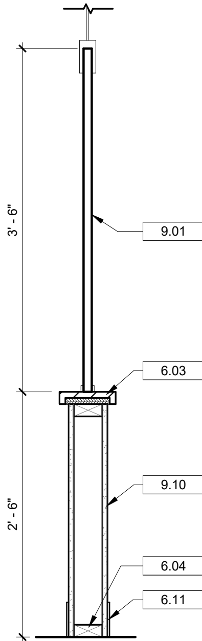
6 SECTION AT TYPICAL KNEE WALL COUNTER A11.02 1" = 1'-0"
